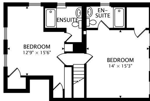
HOUSE 2 SECOND 706 sq ft
